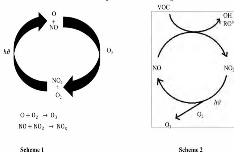
Figure 1. Chemistry of NO x and VOCs towards formation of Ozone in the environment.
