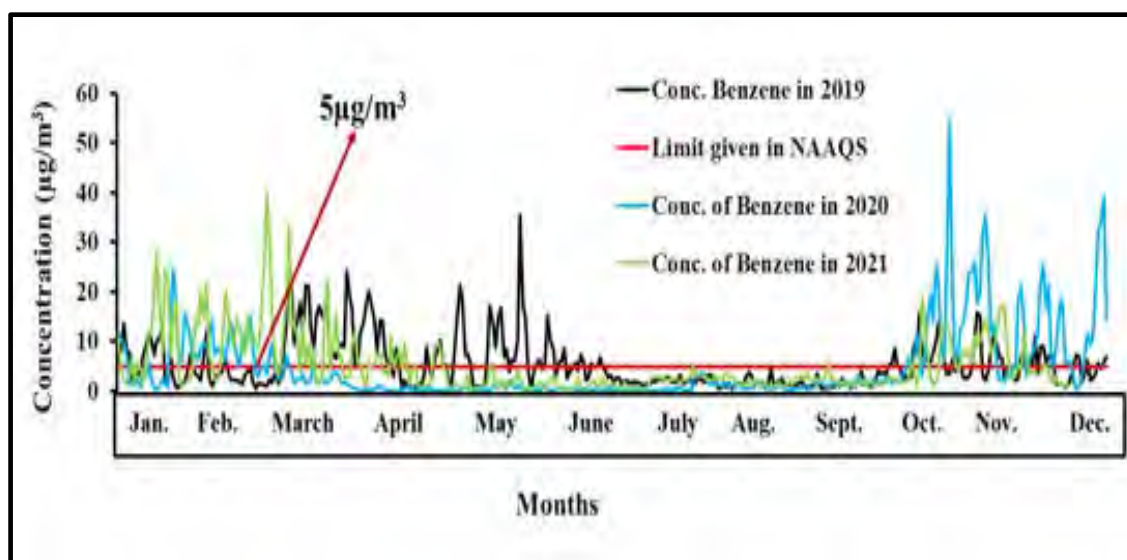
Figure 6. Monthly concentration of benzene from 2019-2021.
